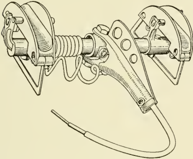
Fig. 3. Slide Contact of Schiemann Current Collector
